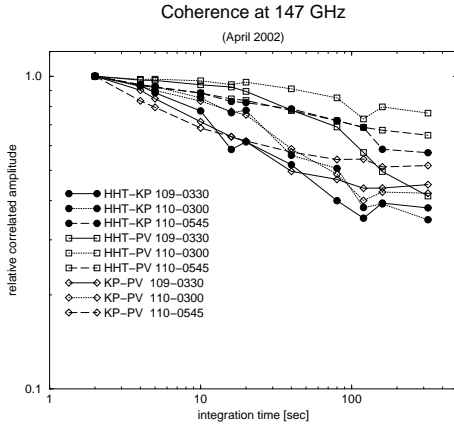
Fig. 1. Normalized correlated visibility amplitude plotted versus coherent integration time for the 3 different baselines and for 3 different times (dd-hhmm). The coherence varies with time and depends mainly on atmospheric conditions. Typically, a 10–20 % amplitude loss is reached after 10 seconds.
